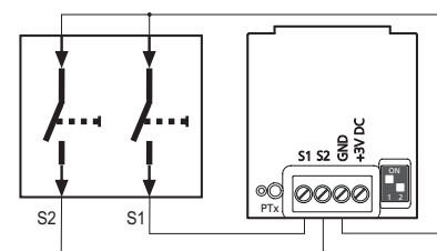
Button connection
