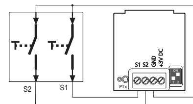
Switch connection
